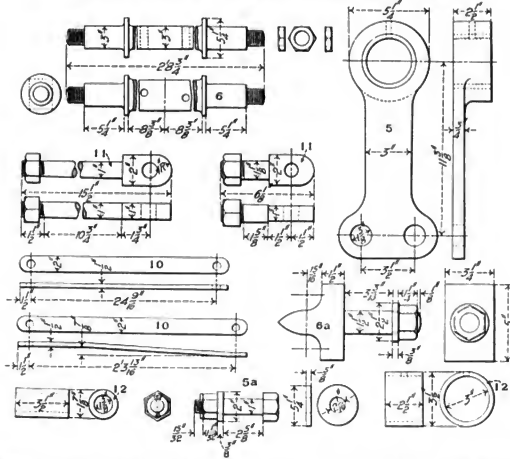
Figs. 3436-3461. Details of Radial Trailing Truck for Atlantic (1-1-2) Locomotive. Pennsylvania Railroad.
